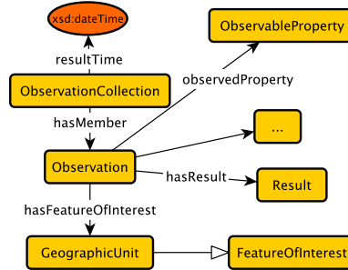
Fig. 5: Using time as the aggregator in SOSA extension
