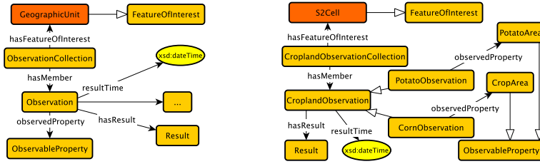
(a) Using geographic unit as the aggregator in SOSA extension. (b) Example of using geographic unit as the aggregator.
