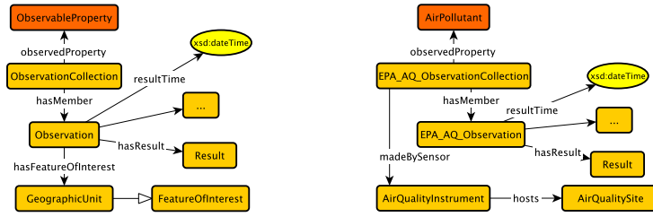
(a) Using observable property as the aggregator in SOSA extension. (b) Example of using observable property as the aggregator.
