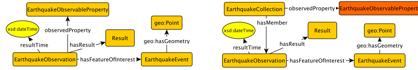
(a) Only using observation to model earthquakes. (b) Using observable property as the aggregator to model earthquakes.
