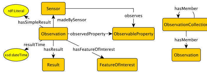
Fig. 1: A top-level, simplified schema diagram for the SOSA ontology (left) and its extension on observation collection (right).
