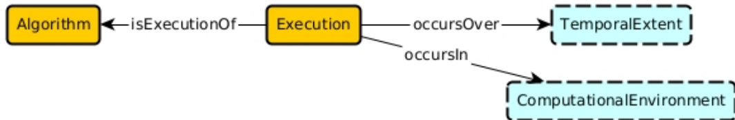
Figure 3: A visual representation of our Algorithm example. The graphical syntax is the same as in Figure 1. Note the correspondences between it and the figure above.
