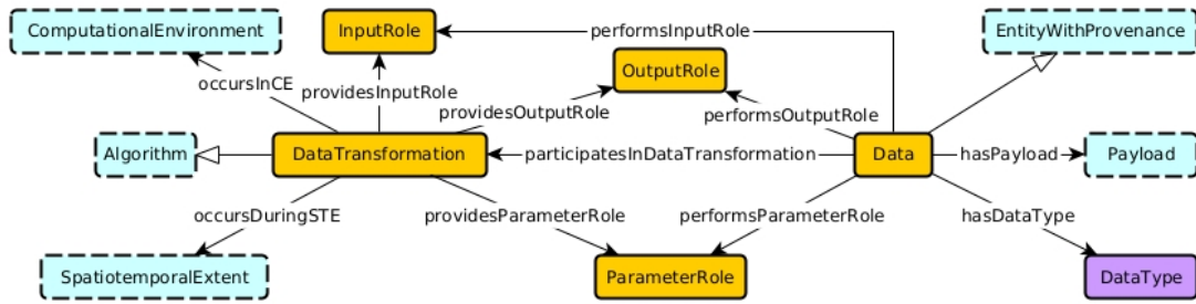
Figure 1: The schema diagram for the Data Transformation Ontology Design Pattern (ODP). Gold boxes represent concepts that are central to the pattern. Blue boxes with dashed borders are interfaces to other patterns or represent concepts with significant complexity, but outside the scope of this pattern. Purple boxes represented controlled vocabularies, which simply means they are comprised of a finite set of individuals. Black-filled arrows represent object or data properties; and open arrows represent subclass relationships.
