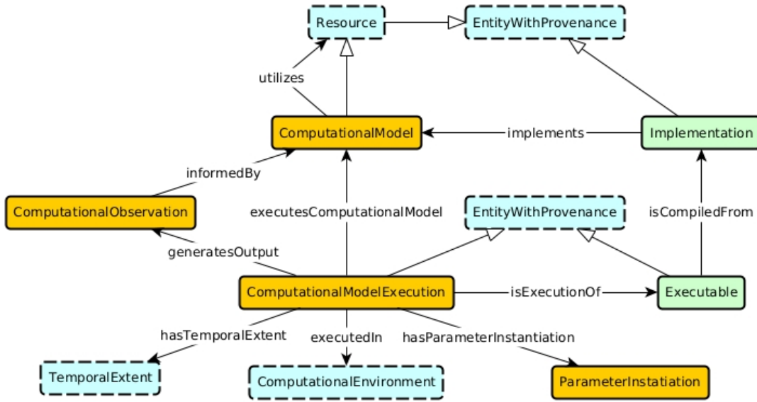
Figure 4: The schema diagram for the Computational Observation ODP. It uses the same graphical syntax as in Figure 1.
